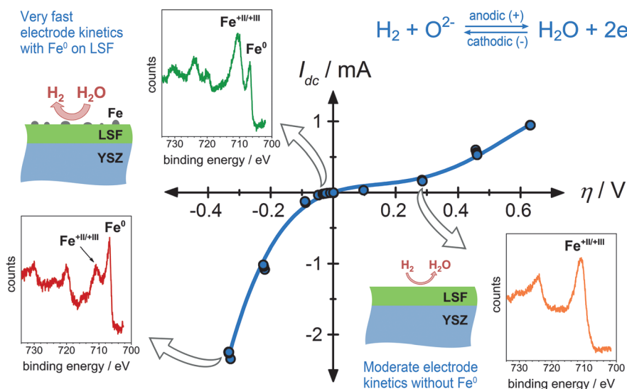
Figure 2. Current–overpotential curve ( I_{\text{dc}} vs. \eta ) of LSF in a humid reducing atmosphere (0.25 mbar H 2 + 0.25 mbar H 2 O). The symbols represent measured values; the line is not a fit but a guide for the eye. The reaction proceeding on the surface of the LSF working electrode is given top right. For selected points of the curve (indicated by arrows), Fe 2p XPS spectra are shown as insets. The sketches indicate the situation for the LSF surface and the resulting reactivity, respectively.
