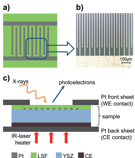
Figure 1. a) Sketch and b) optical micrograph of a sample with thin LSF electrode and buried current collector. c) Sketch (cross section) of a sample mounted for NAP-XPS measurements (WE—working electrode, CE—counter electrode).
